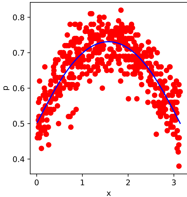
True p with sample data.
