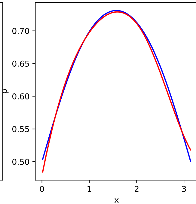
True v. fitted p
